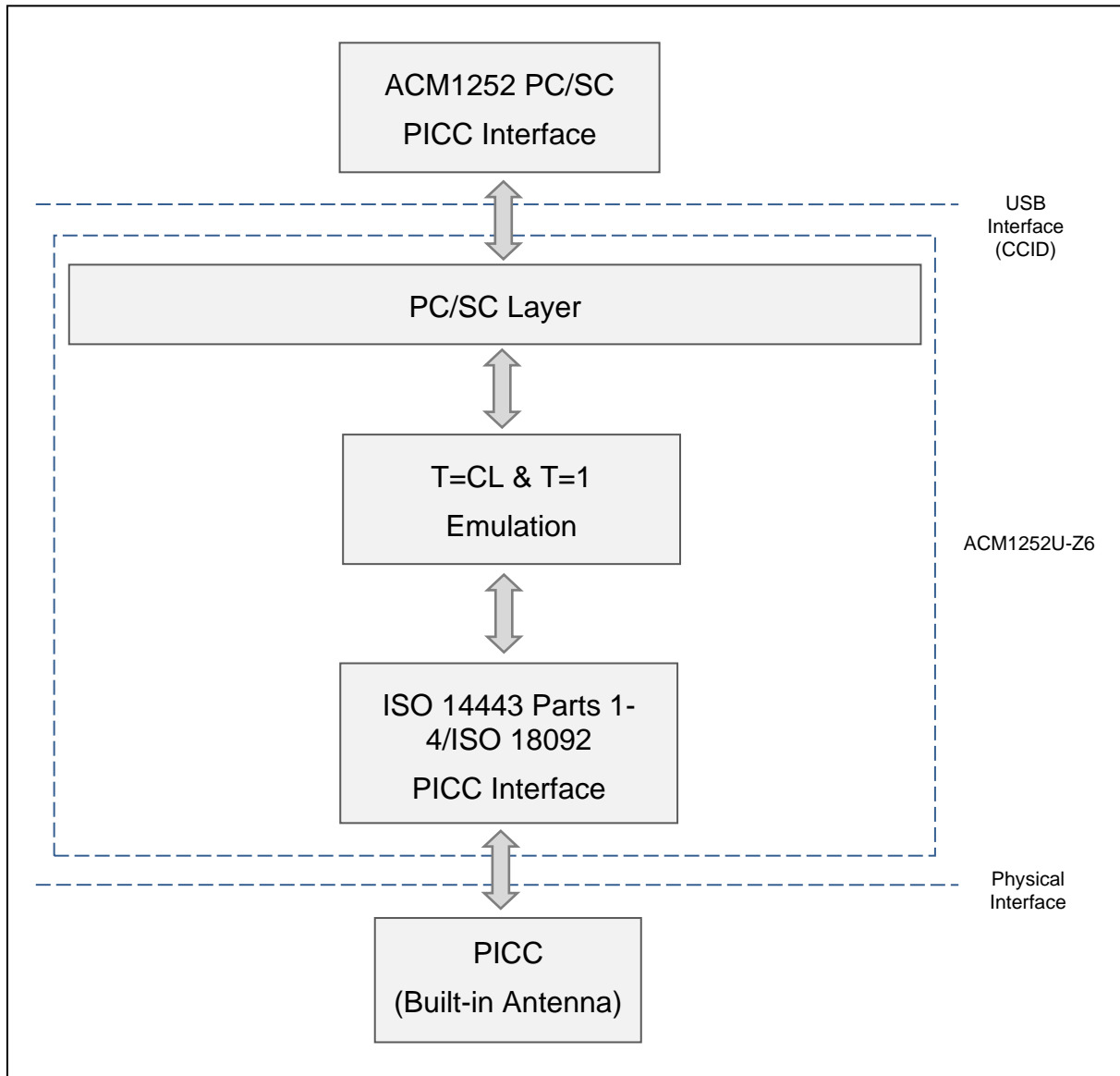
Figure 1: ACM1252U-Z6 Architecture
